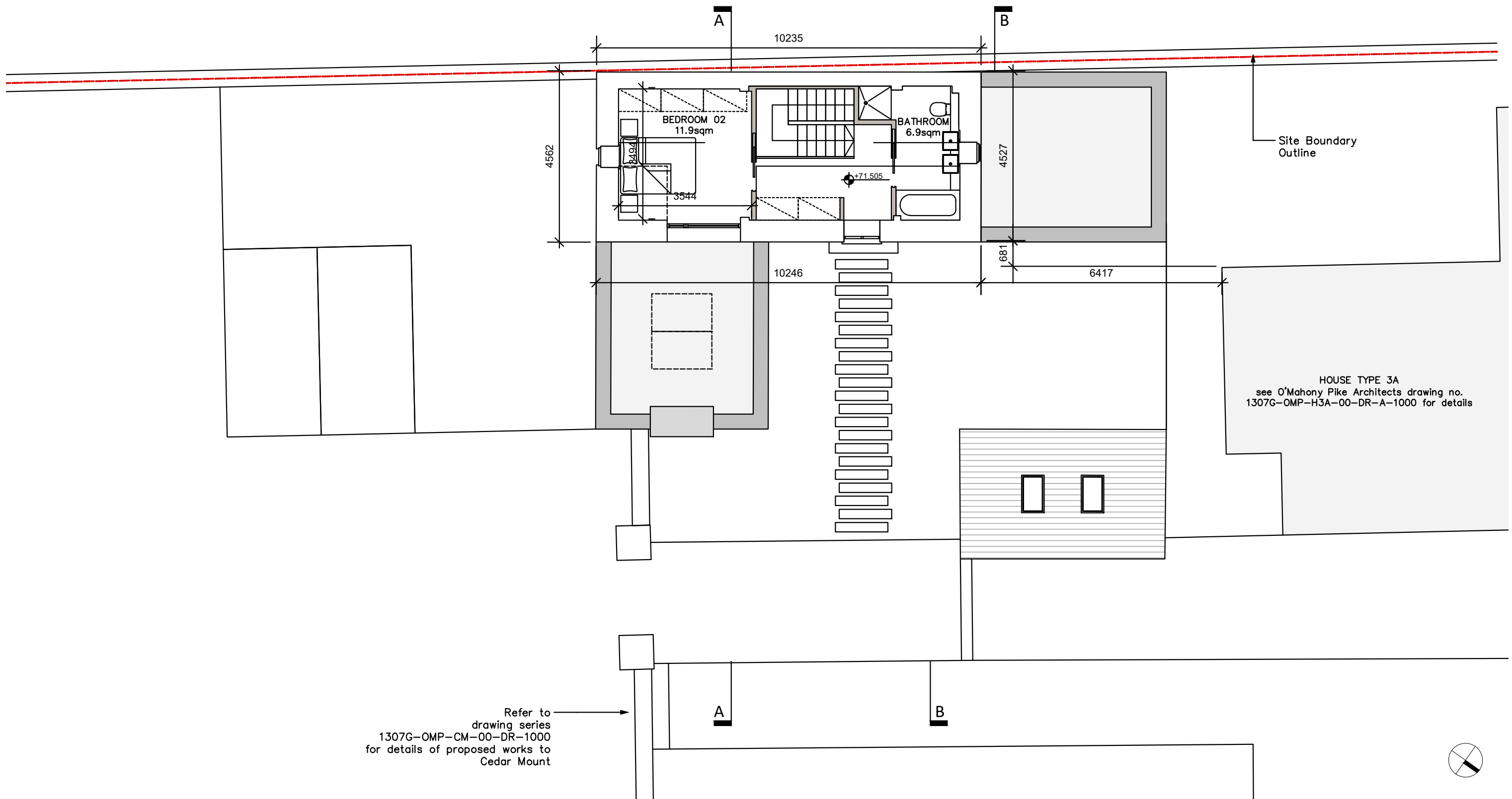
Coach House, Proposed First Floor Plan
